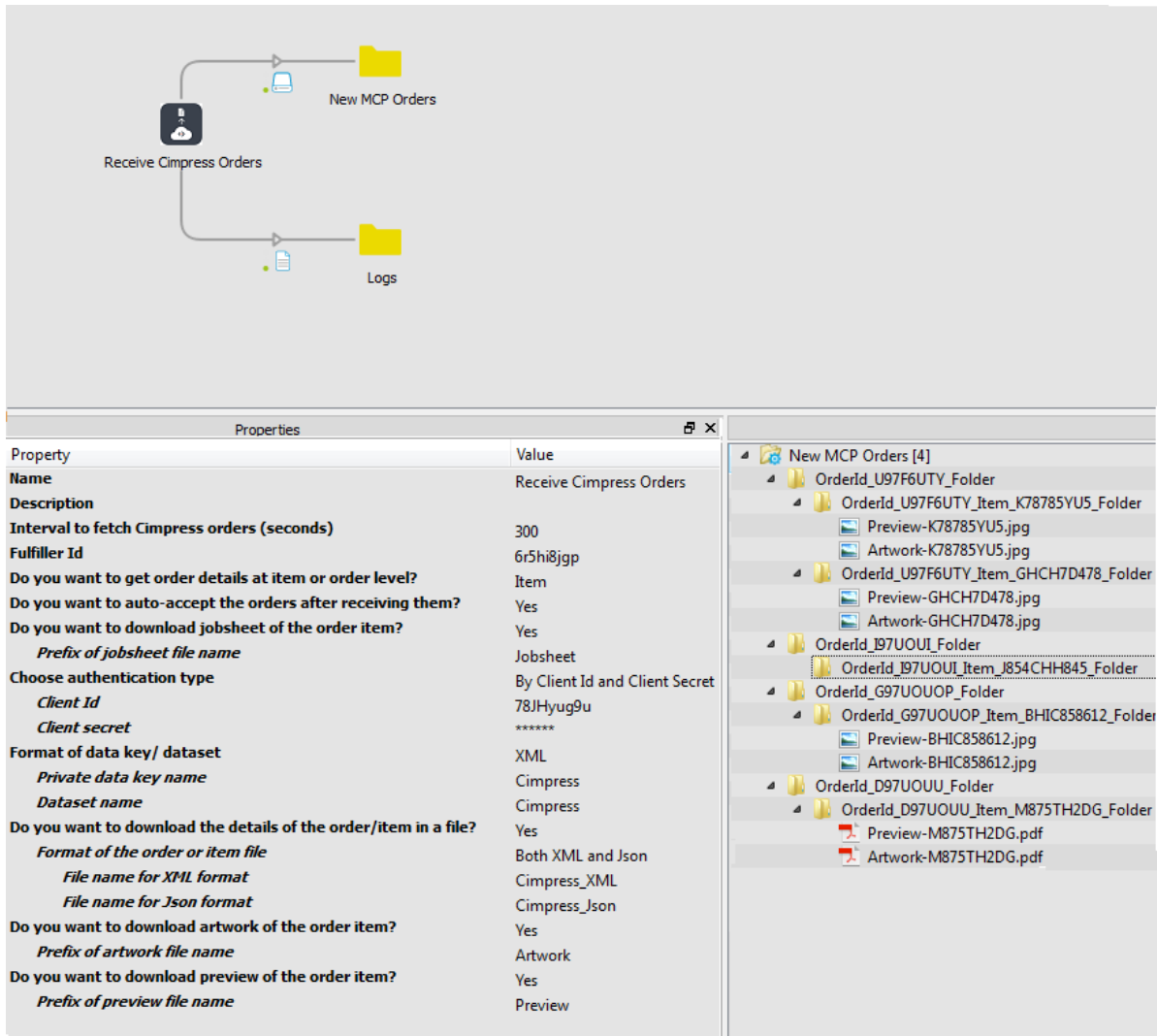
Fig 2: Flow with authentication by Client Id and Client Secret
